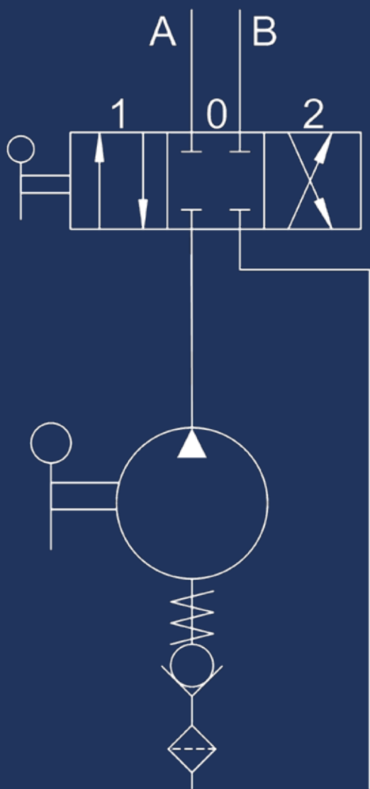
HYDRAULIC DIAGRAM
